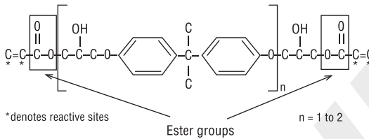
Figure 16 - Idealised Chemical Structure of a Typical Epoxy Based Vinylester
